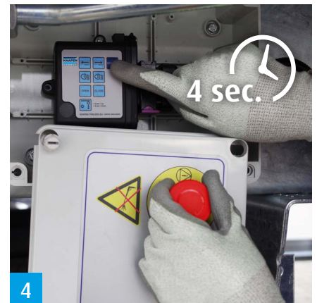
Press and hold the ENABLE button on the receiver and deactivate the emergency button. Release the ENABLE button after 4 seconds
