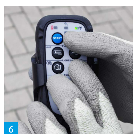
Press 3 random buttons simultaneously on the remote control. The remote control and the receiver are now paired and ready for use
